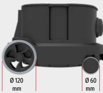
Extra-large rubberised wheels and castors.
