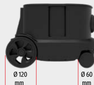
Extra-large wheels and castors ensure a high level of agility and stability.
