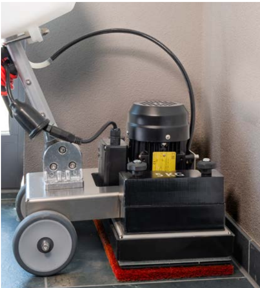
Rectangular pads: perfect edge and corner cleaning without manual reworking
